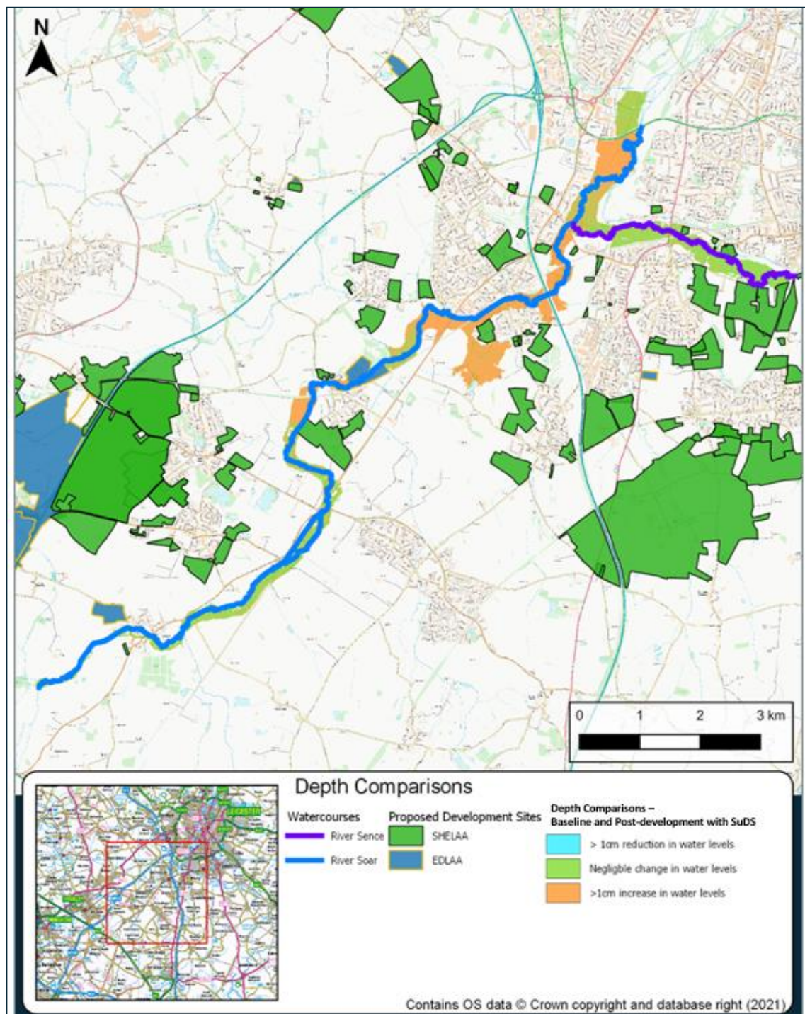
Figure 7-18 below shows that the impact on flood flows in the River Soar and River Sence model as a result of the proposed development in Blaby district. With the implementation of necessary SuDS mitigations to maintain the peak discharges at existing levels, most of the model domain shows no significant changes in flood extent and depth ( \pm 1\text{cm} ), and large parts of the results outside this bracket shows no more than a 5cm increase in flood depths.
