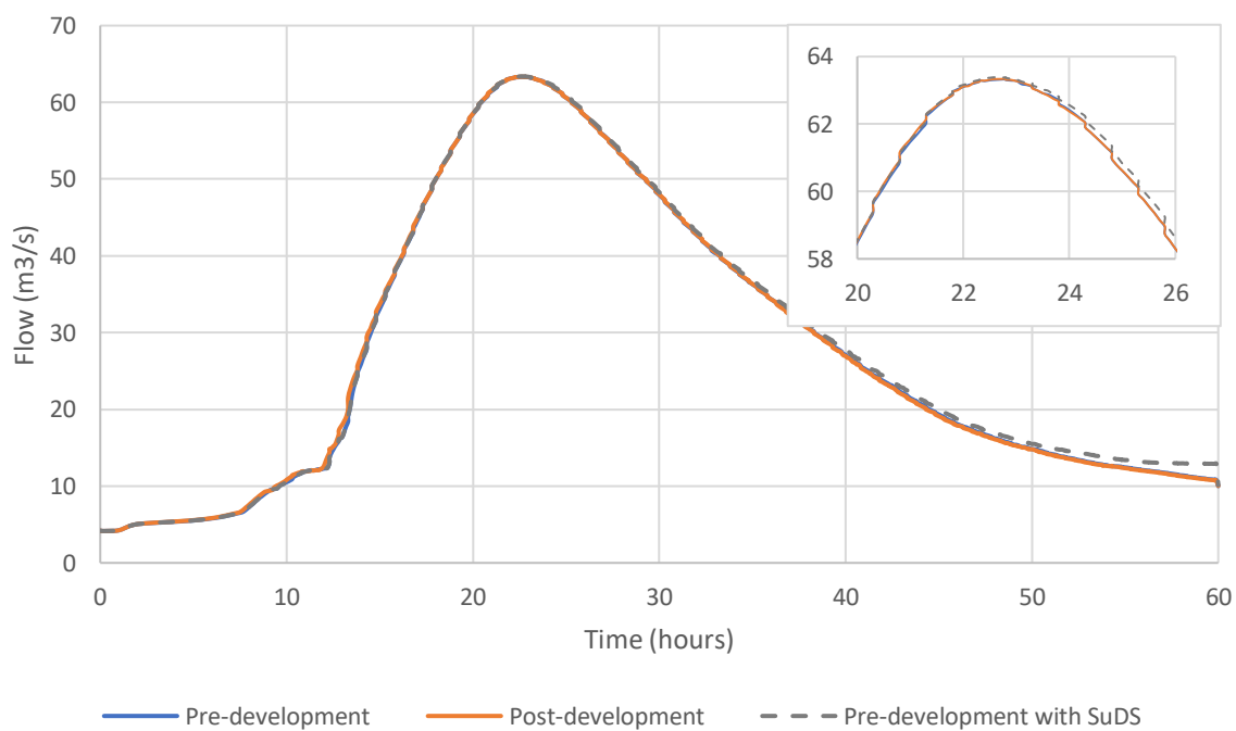
Figure 7-16: Pre-, Post-development and SuDS Hydrographs in the Sence catchment hydrological model results.
