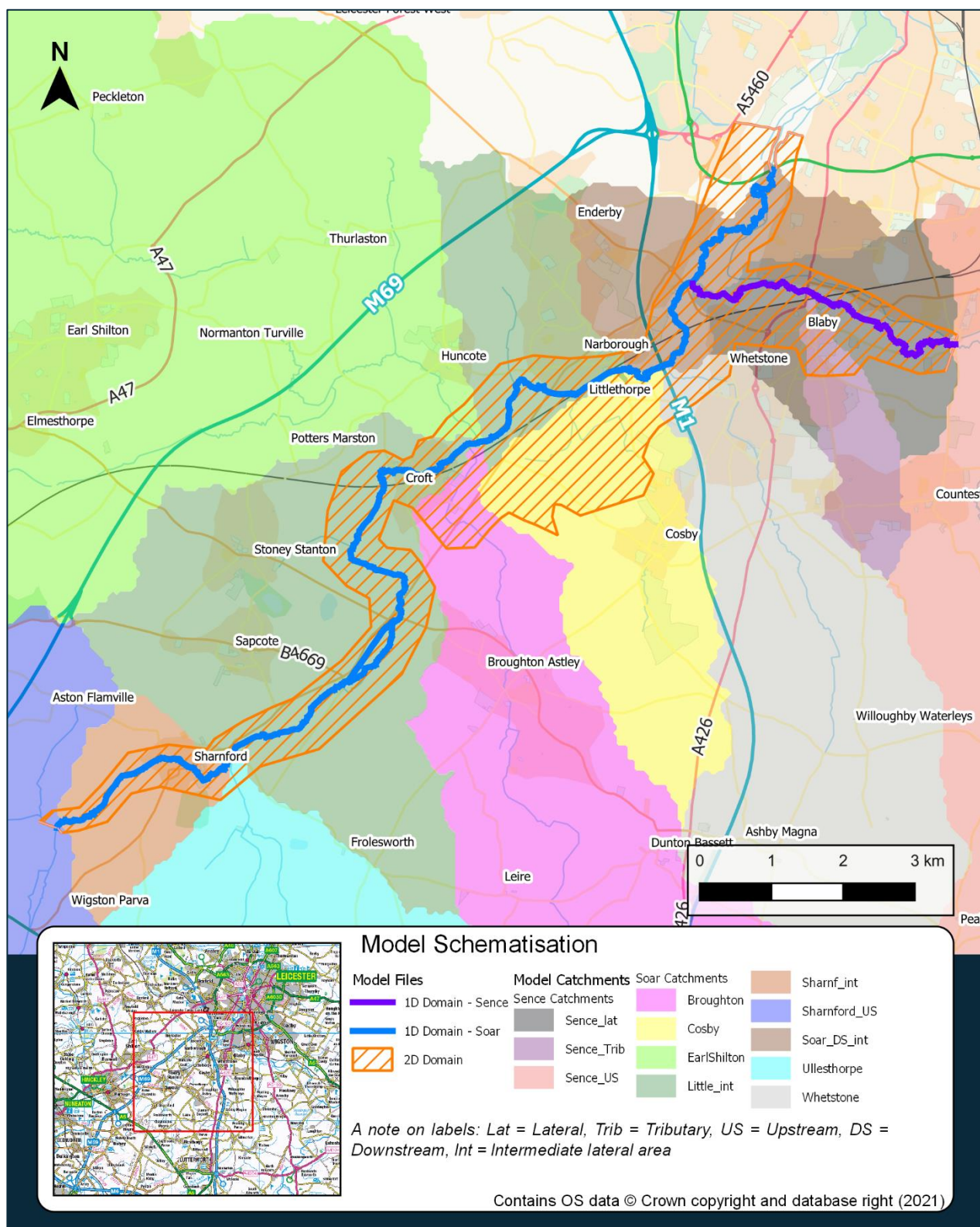
Figure 7-3: Jacobs' River Soar 2018 Model
