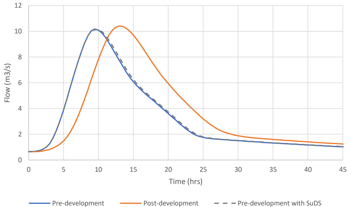
Figure 7-11: Pre- and post-development and SuDS hydrographs in the Lubbesthorpe Brook catchment
